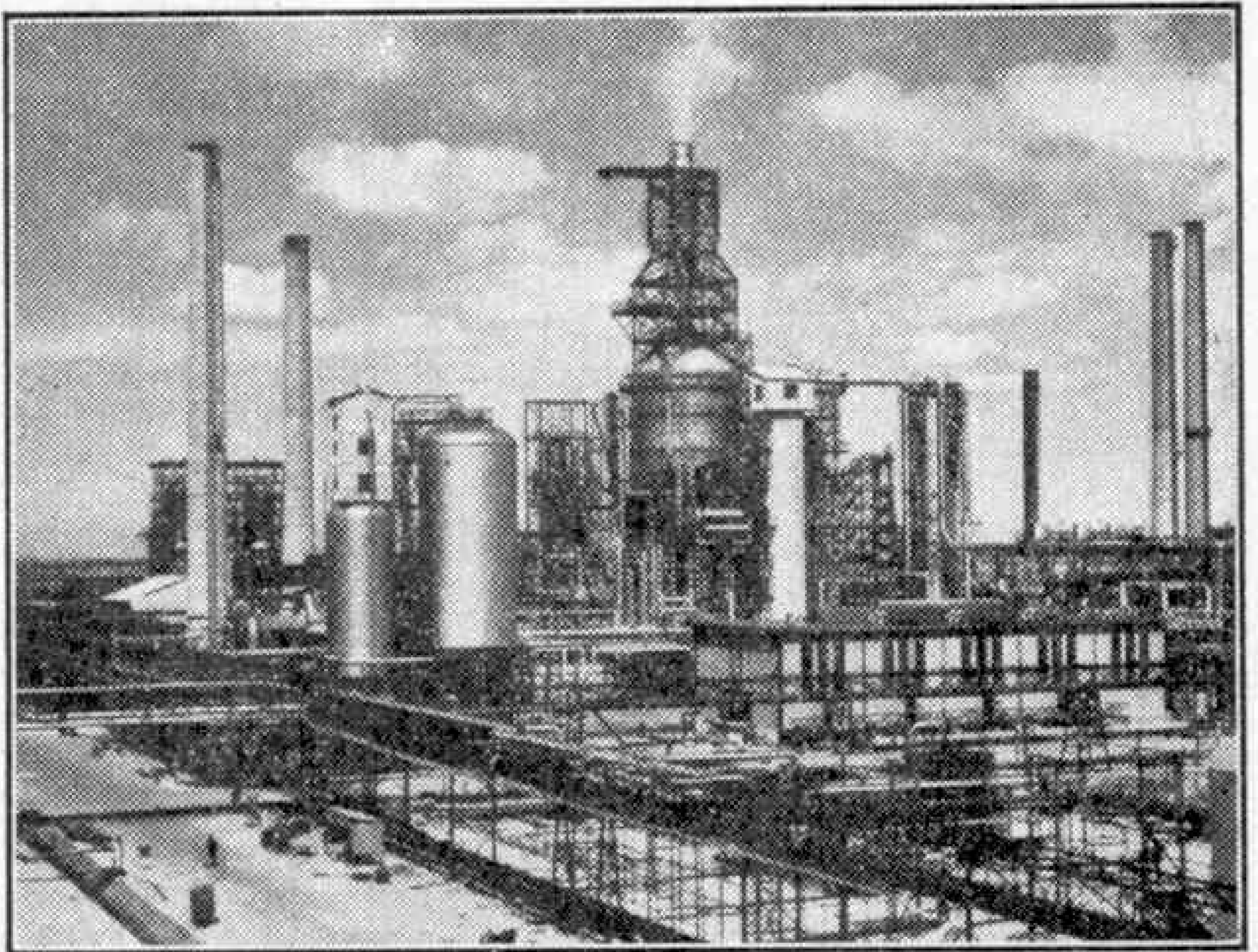
The cat-cracker at the Pernis Refinery. The rectangular structure is the catalyst regenerator, and the fractionating column is on its right. On the left is the 196 ft. chimney stack of the furnace.
