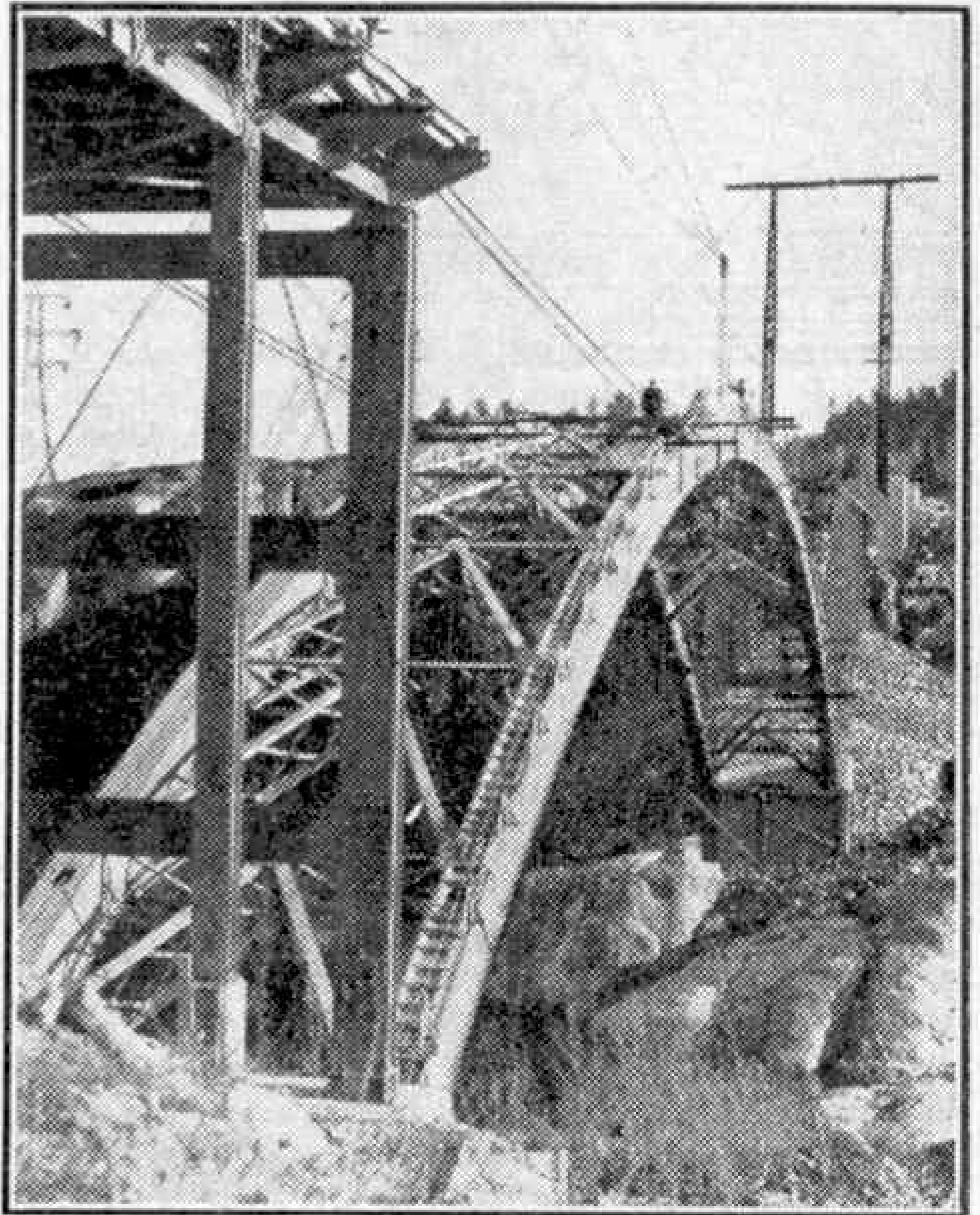
The world's first aluminium highway bridge under construction at Arvida. The arch has been completed and is ready for the erection of the posts that support the deck structure.
