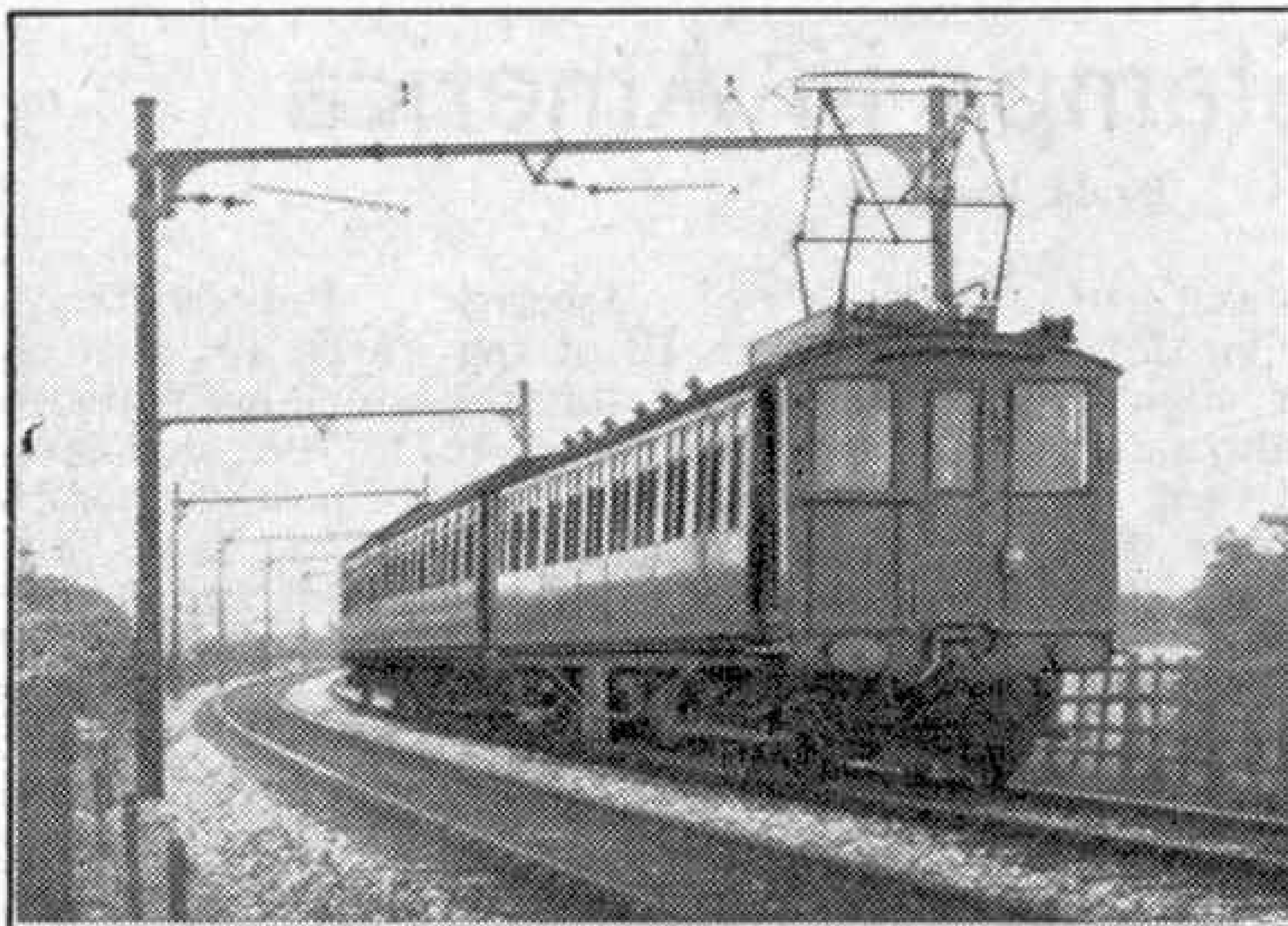
A typical scene on the Morecambe-Heysham line when operated on the 6,600-volt overhead electrification system, now discontinued. Photograph by W. S. Garth.
